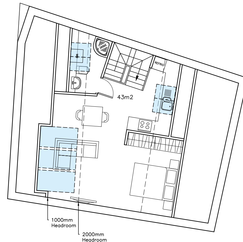
Proposed Third Floor Plan
