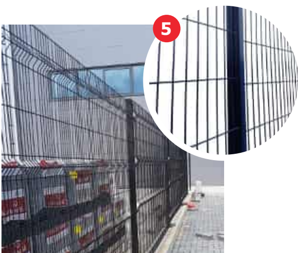
Fencing & Enclosures: 2.4m High Welded Mesh Panel in Black (5)
