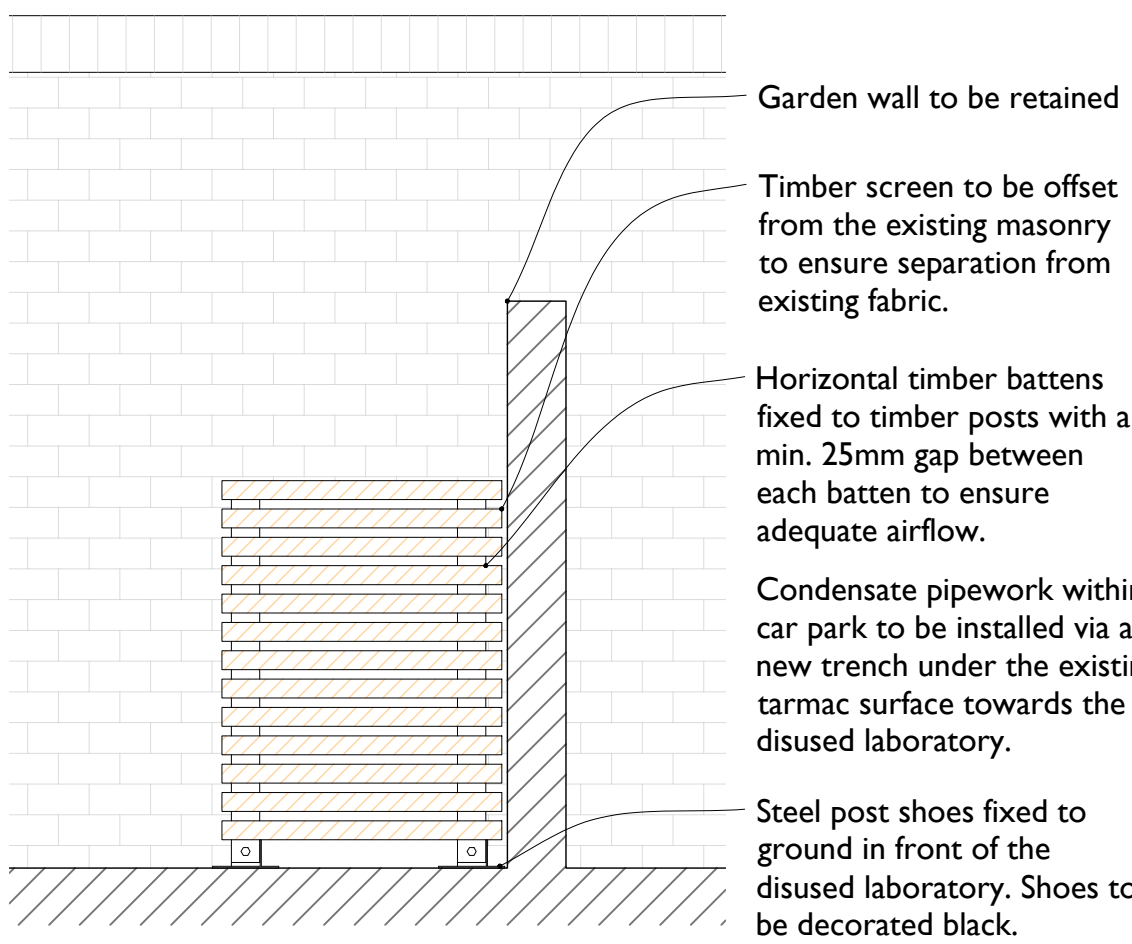
Side Elevation of Proposed Timber Screen 1:20 at A1
