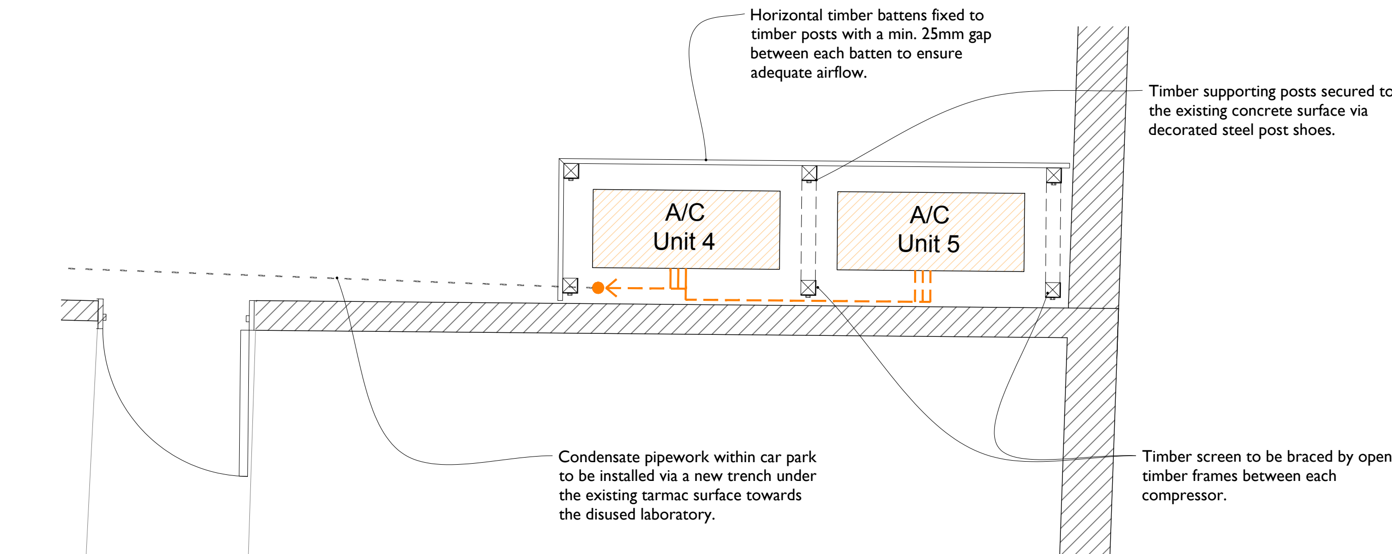
Detail Layout of the Condensers and Proposed Timber Screen 1:20 at A1
