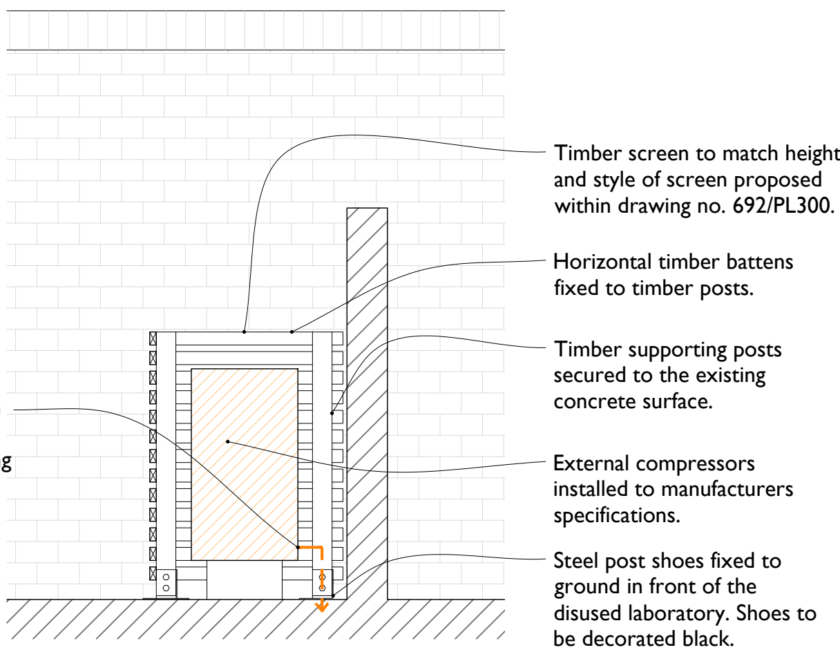
Section Through Timber Screen 1:20 at A1
