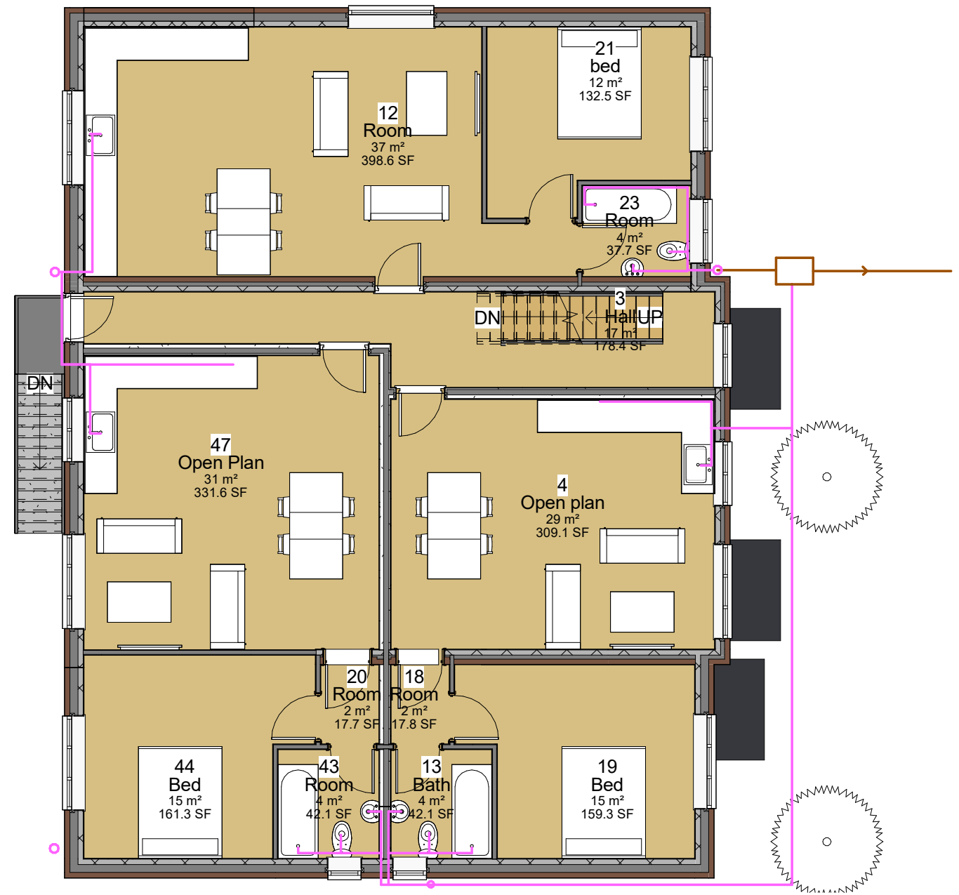
2 First Floor Plan 1 : 100
