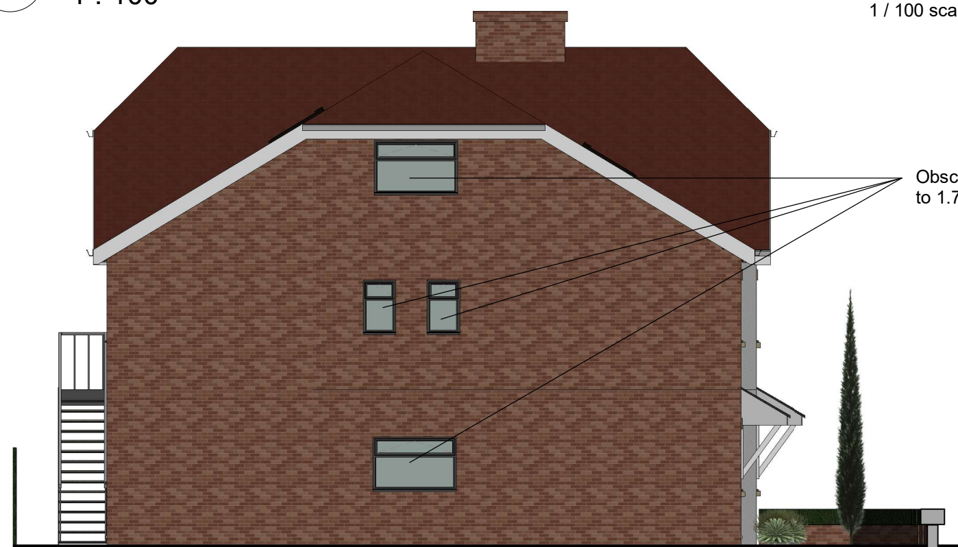
3 South Elevation 1 : 100
