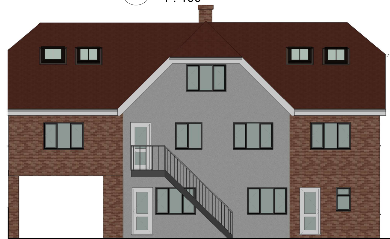
4 West Elevation 1 : 100
