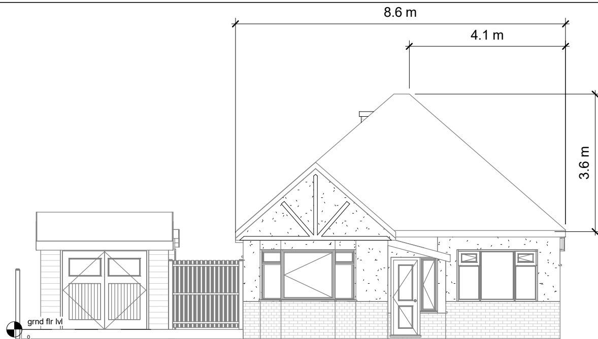
Existing Elevation-Front
