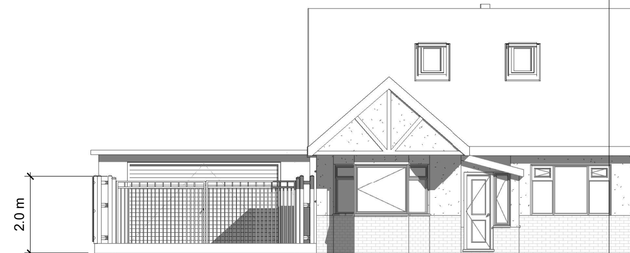
Proposed Elevation-Front
