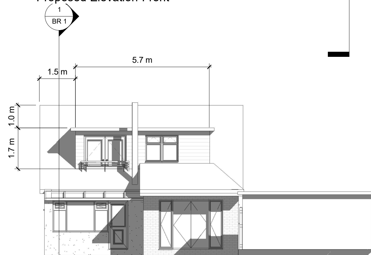
Proposed Elevation-Rear
