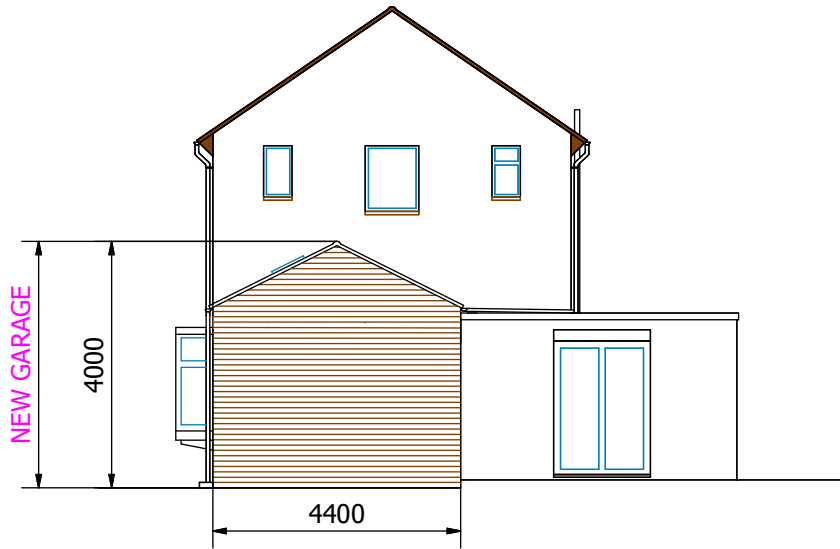
East Elevation (view from Monkwood Close)
