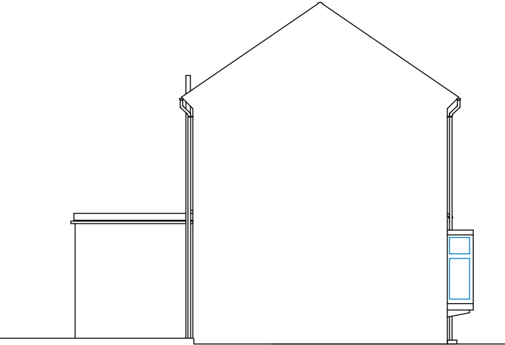
West Elevation (view from 25 Rownhams)
