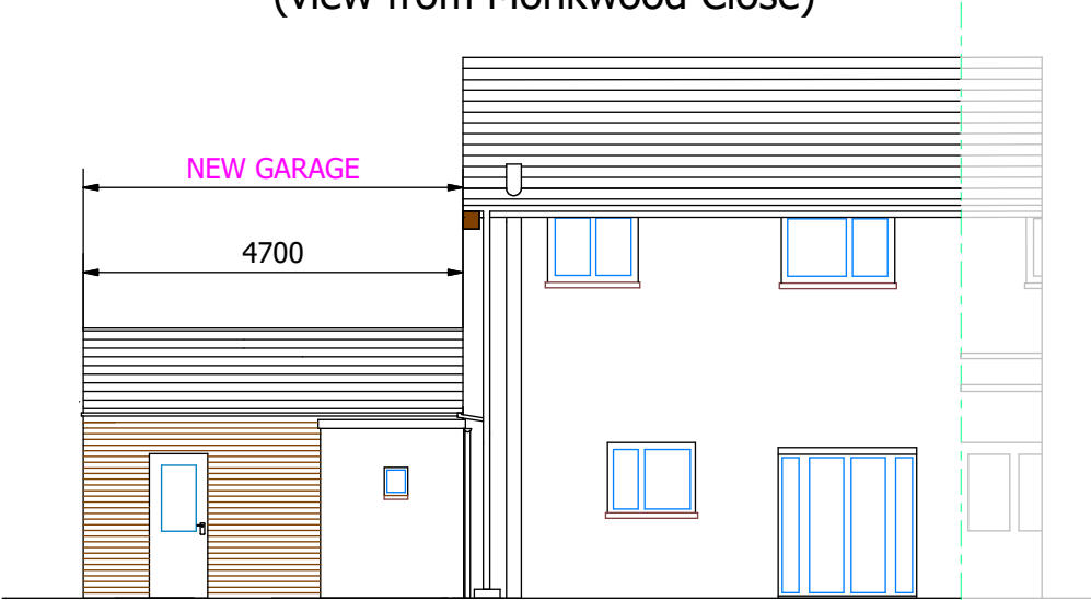
North Elevation (rear of property)
