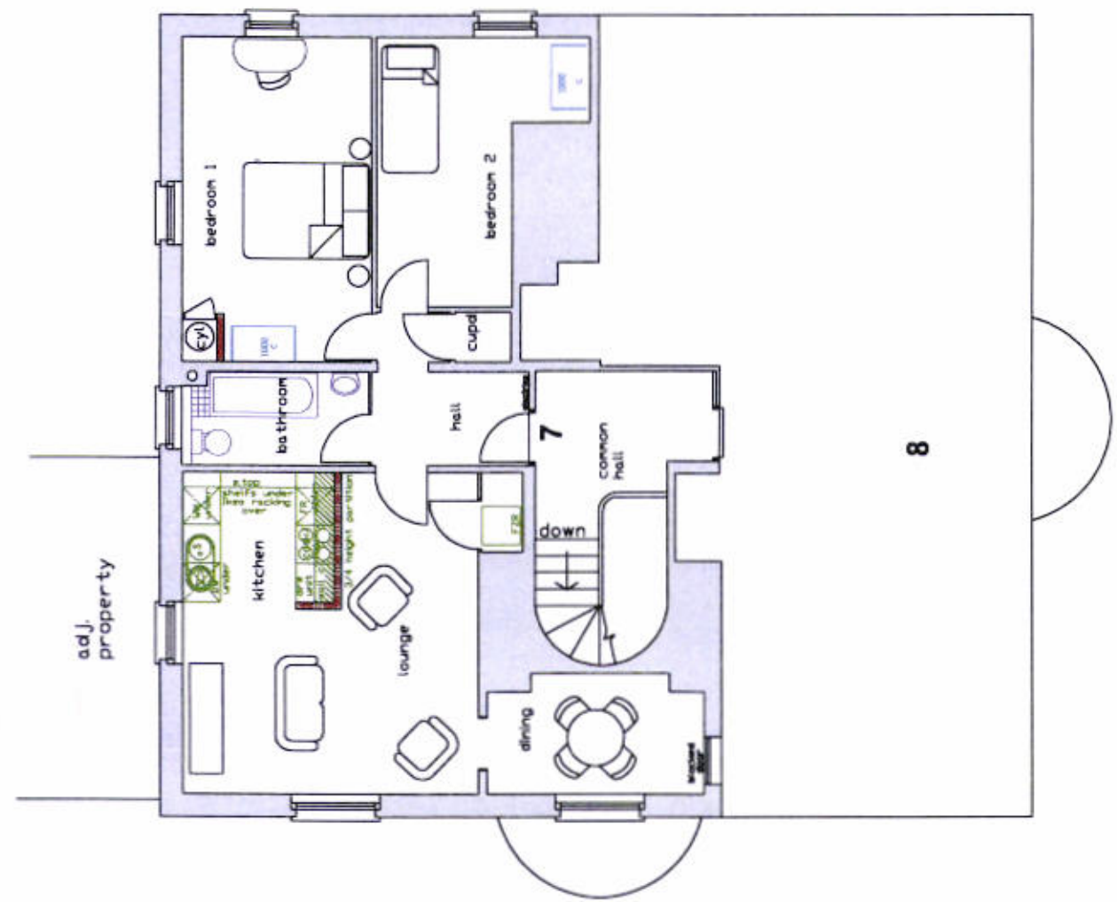
SECOND FLOOR PLAN PROPOSED
