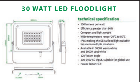
E FIVE X LED FLOOD LIGHTS SIZE. 0.23m x 168mm. H.A.G. 6m.
