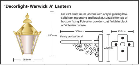
D ONE X BRASS PORTLAND LANTERN SIZE. 0.28m x 650mm. H.A.G. 2m.
