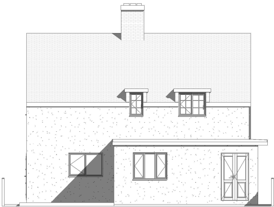
Proposed Elevation-Rear
