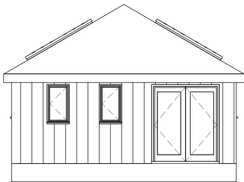
North Elevation
