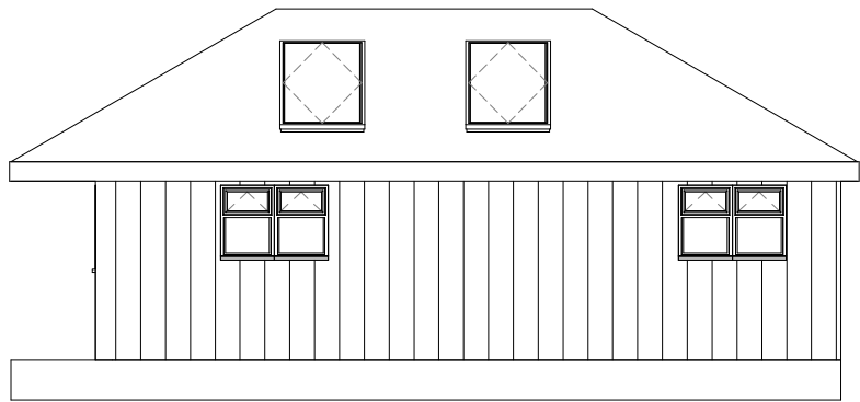
West Elevation
