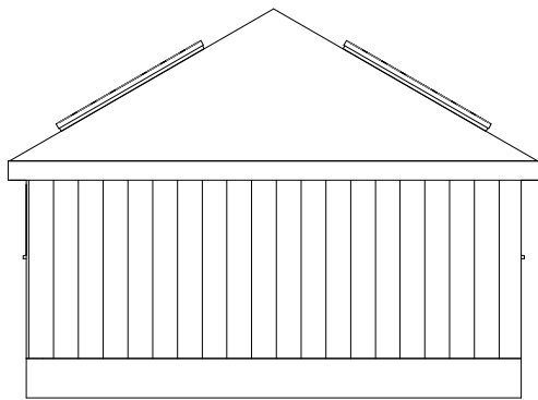
South Elevation
