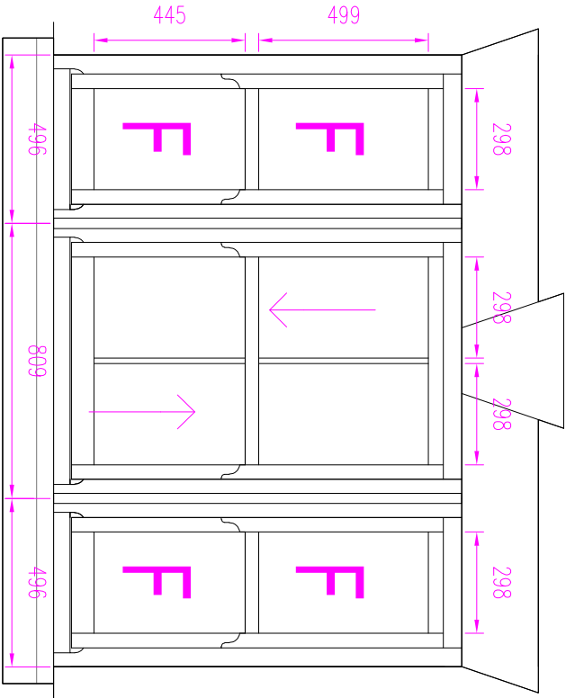
TYPICAL WINDOW ELEVATION (W05 - W06 Similar)
