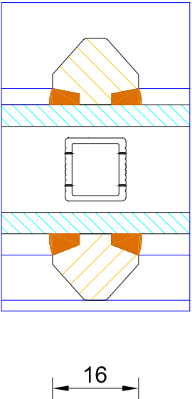
Glazing Bar Detail (1:1 Scale)
