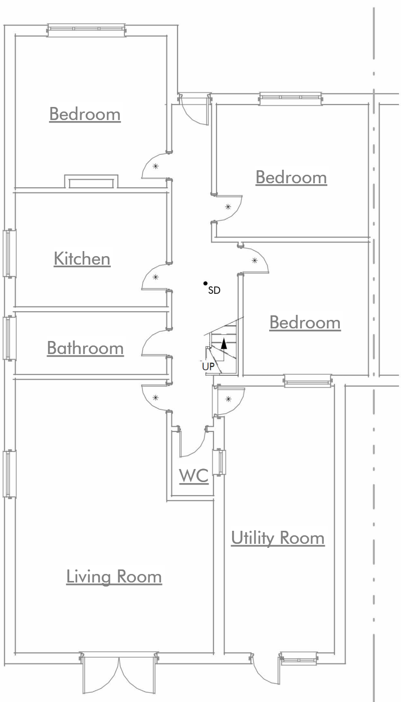
0 - Proposed Ground Floor 1 : 100
