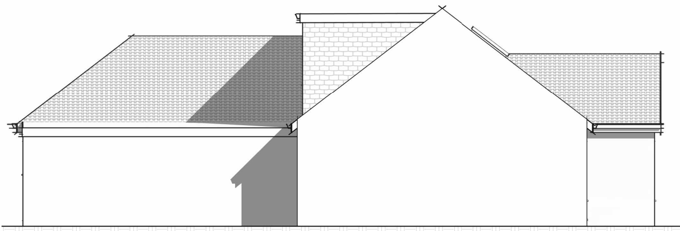
Proposed Side (North) 1 : 100
