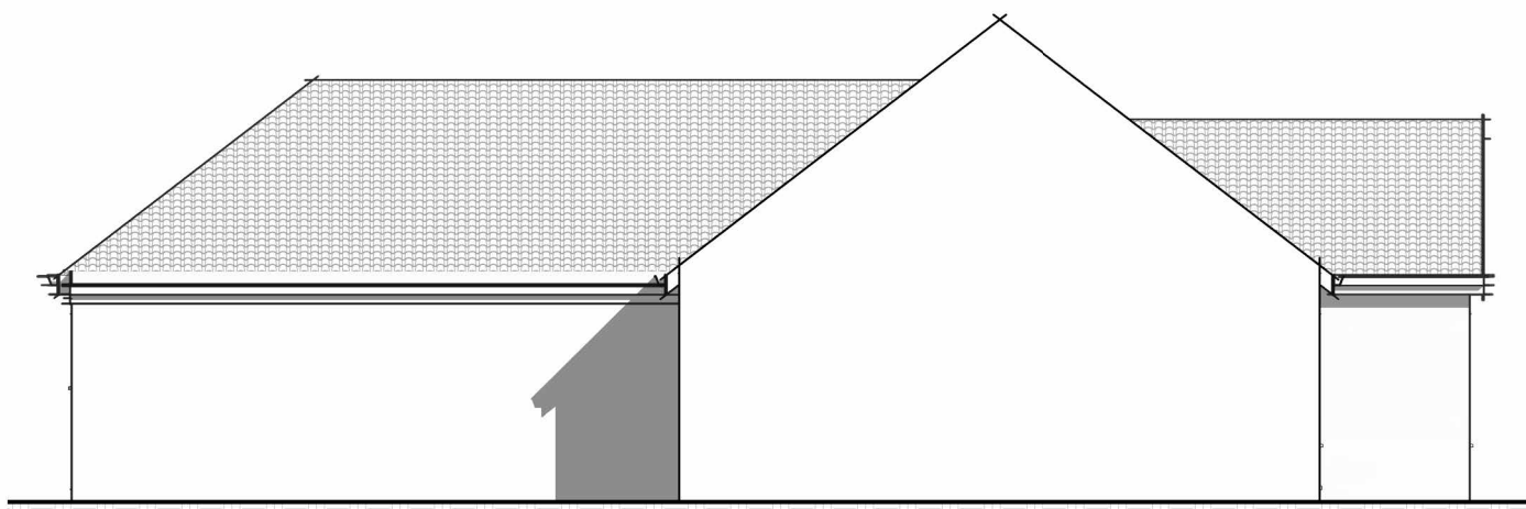
Existing Side (North) 1 : 100
