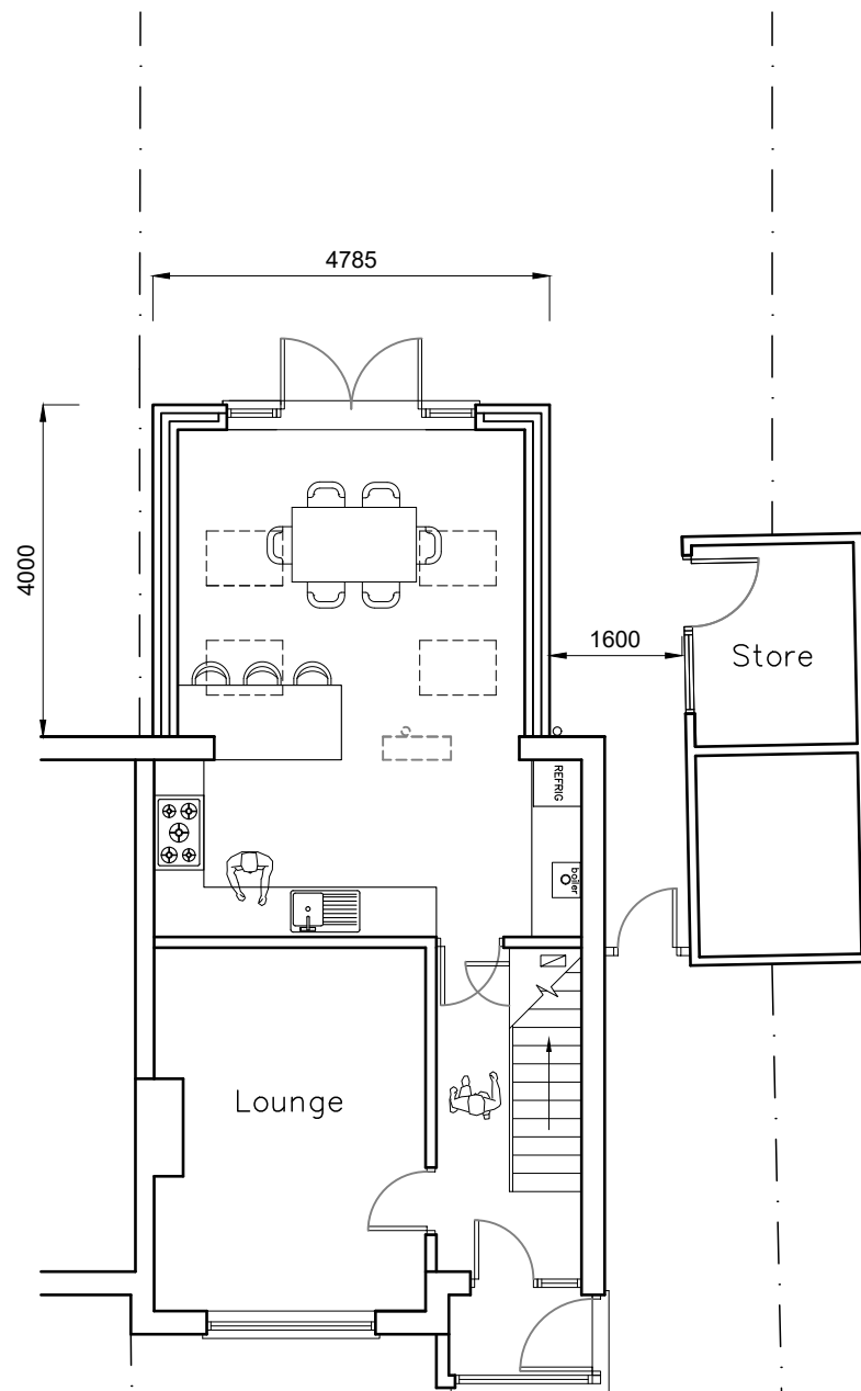
GROUND FLOOR
