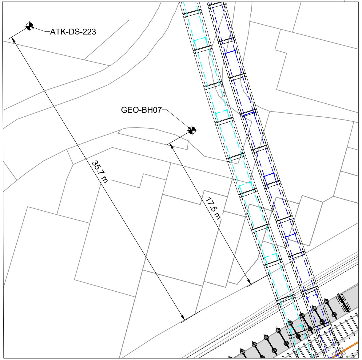
ADDITIONAL BOREHOLES LOCATION DETAIL SCALE 1:250
