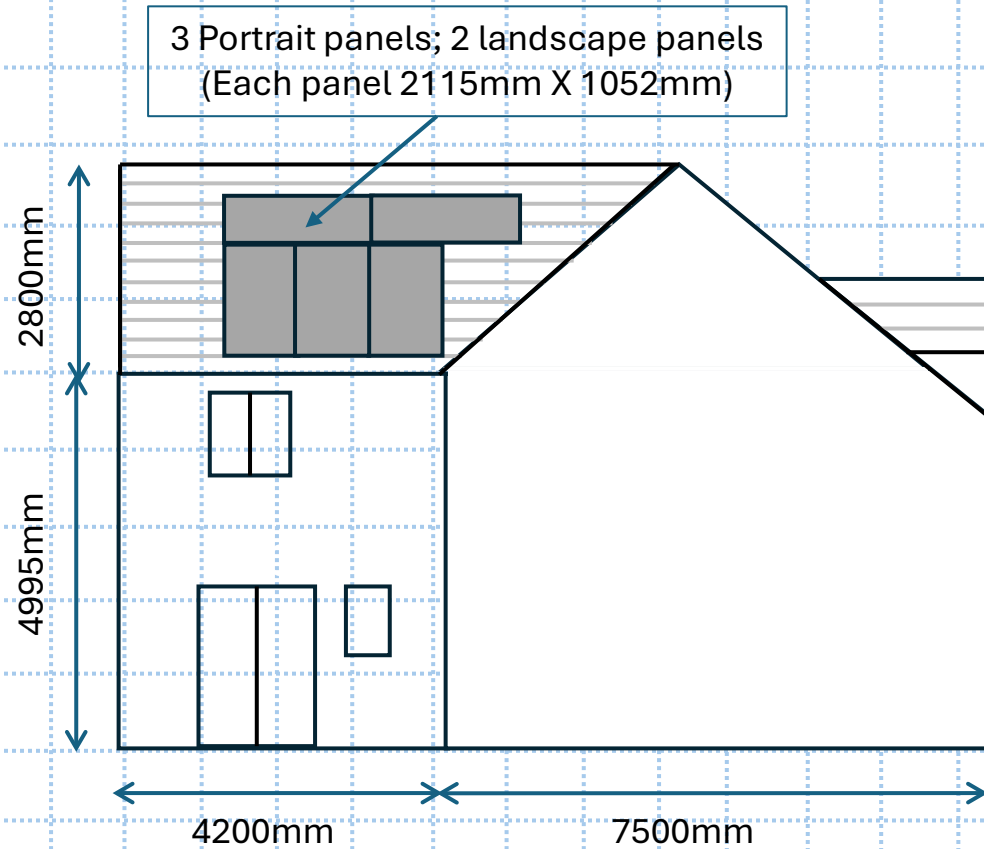
REAR (SOUTHERN) ELEVATION
