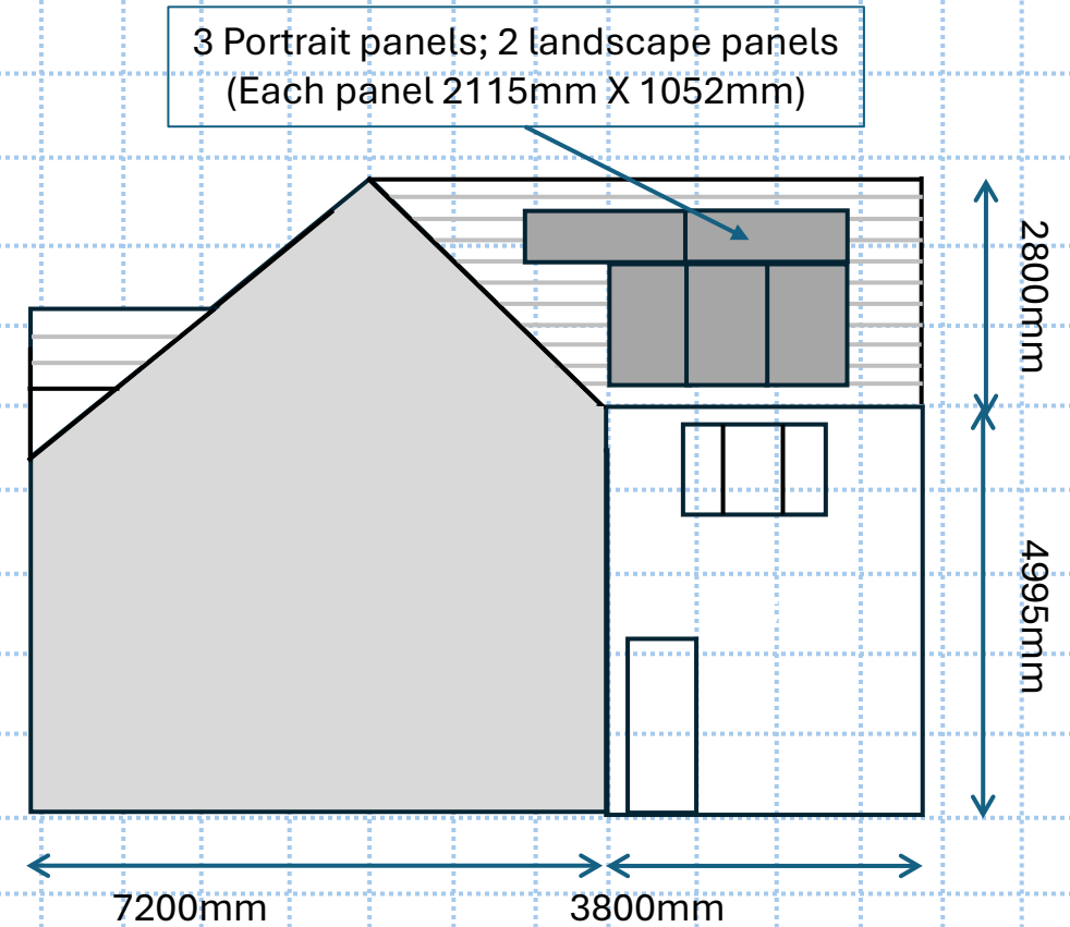
SIDE (WEST) ELEVATION
