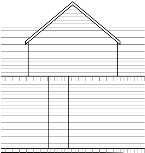
Porch - West Elevation 1:50
