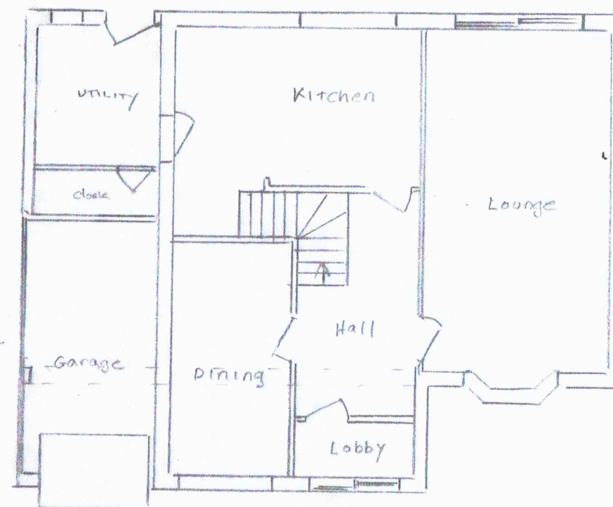
Proposed Floor Plans
