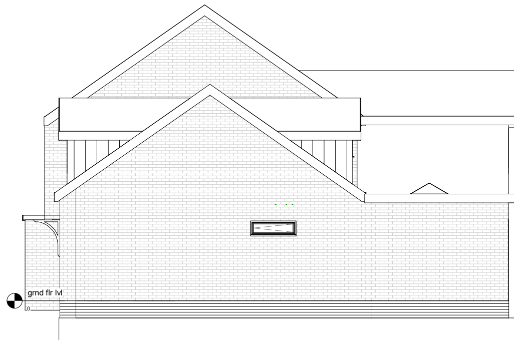
Existing Elevation-Right side
