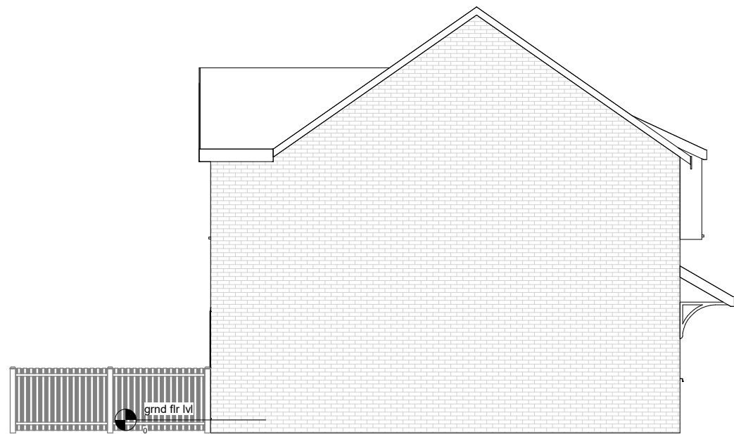
Existing Elevation-Left side
