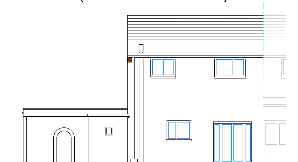
East Elevation (view from Monkwood Close)
