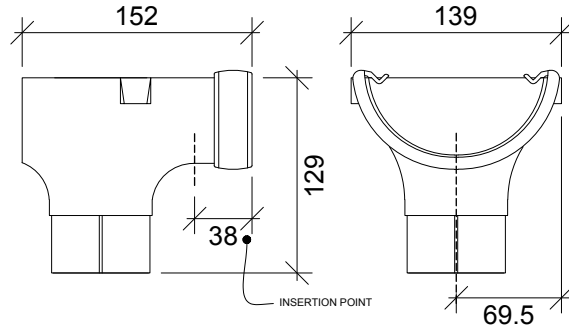
CAST IRON STYLE RAINWATER SYSTEM HALF ROUND 112MM STOPEND OUTLET
