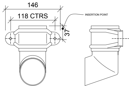
CAST IRON STYLE RAINWATER SYSTEM 68MM ROUND DOWNPIPE SHOE (WITH FIXING LUGS)
