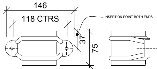
CAST IRON STYLE RAINWATER SYSTEM 68MM ROUND DOWNPIPE AND FITTINGS PIPE SOCKET (WITH FIXING LUNGS)
