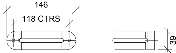
CAST IRON STYLE RAINWATER SYSTEM 68MM ROUND DOWNPIPE AND FITTINGS PIPE CLIP
