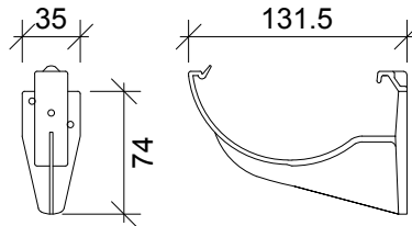
CAST IRON STYLE RAINWATER SYSTEM HALF ROUND 112MM FASCIA BRACKET
