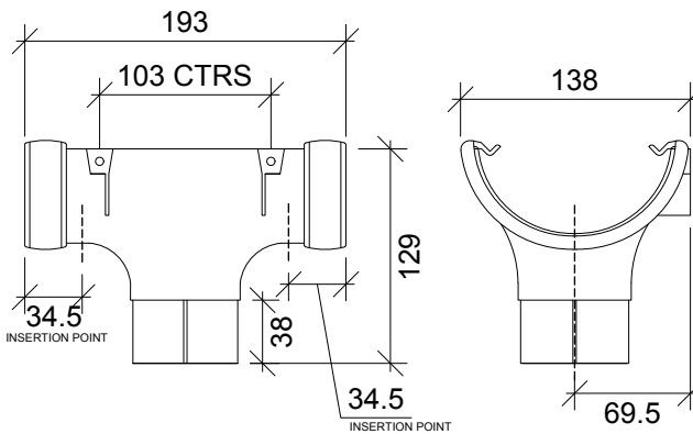
CAST IRON STYLE RAINWATER SYSTEM HALF ROUND 112MM RUNNING OUTLET
