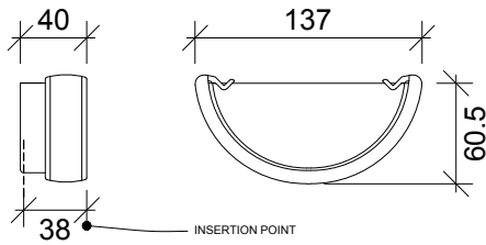
CAST IRON STYLE RAINWATER SYSTEM HALF ROUND 112MM EXTERNAL STOPEND
