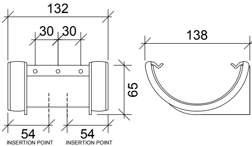
CAST IRON STYLE RAINWATER SYSTEM HALF ROUND 112MM UNION BRACKET
