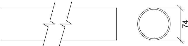
CAST IRON STYLE RAINWATER SYSTEM 68MM ROUND DOWNPIPE
