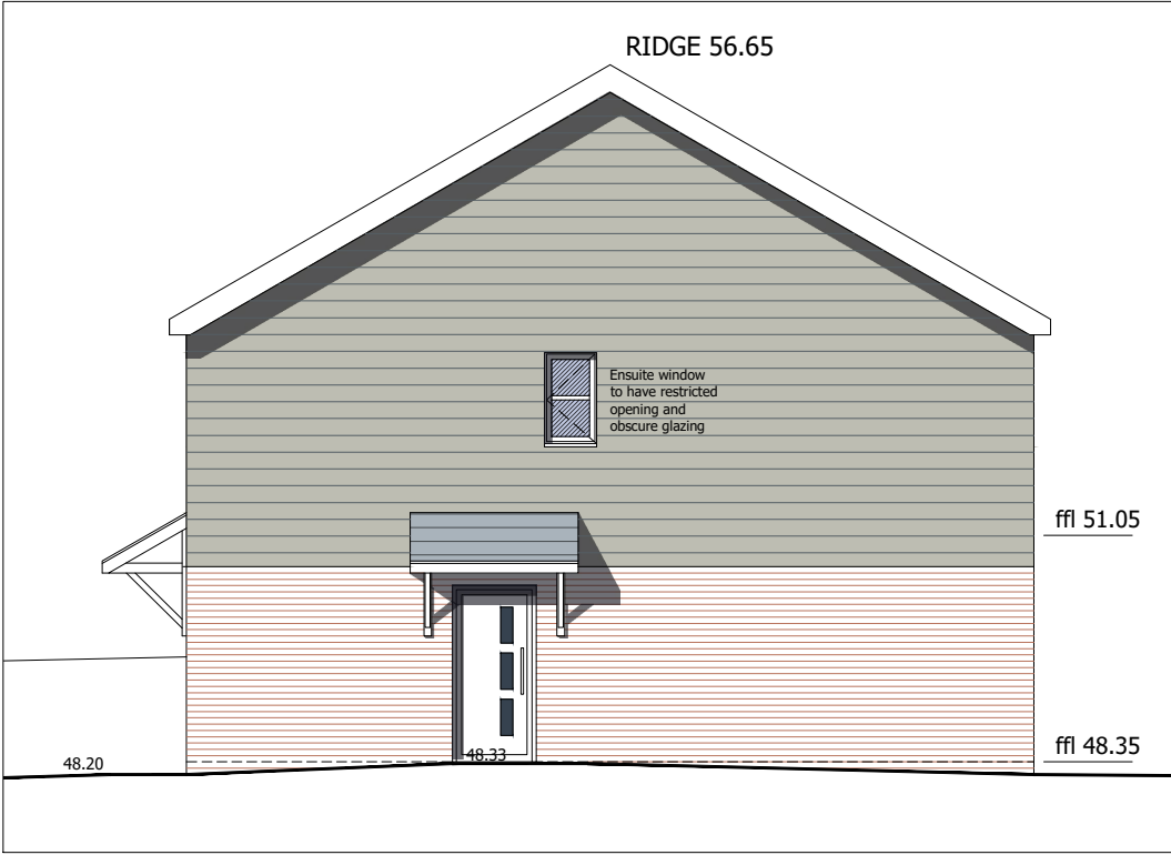
EAST ELEVATION
