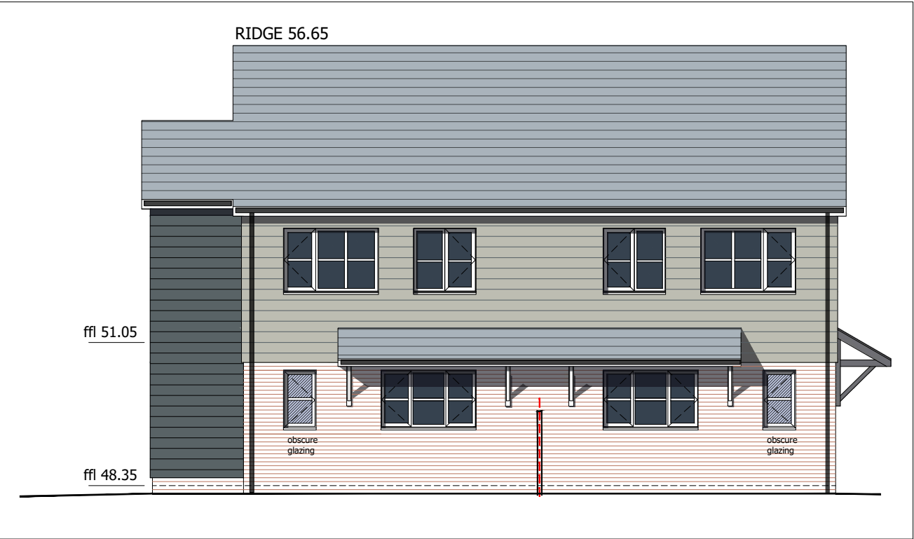
SOUTH ELEVATION
