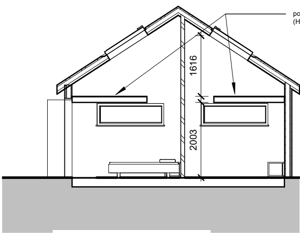
Mezzanine Section
