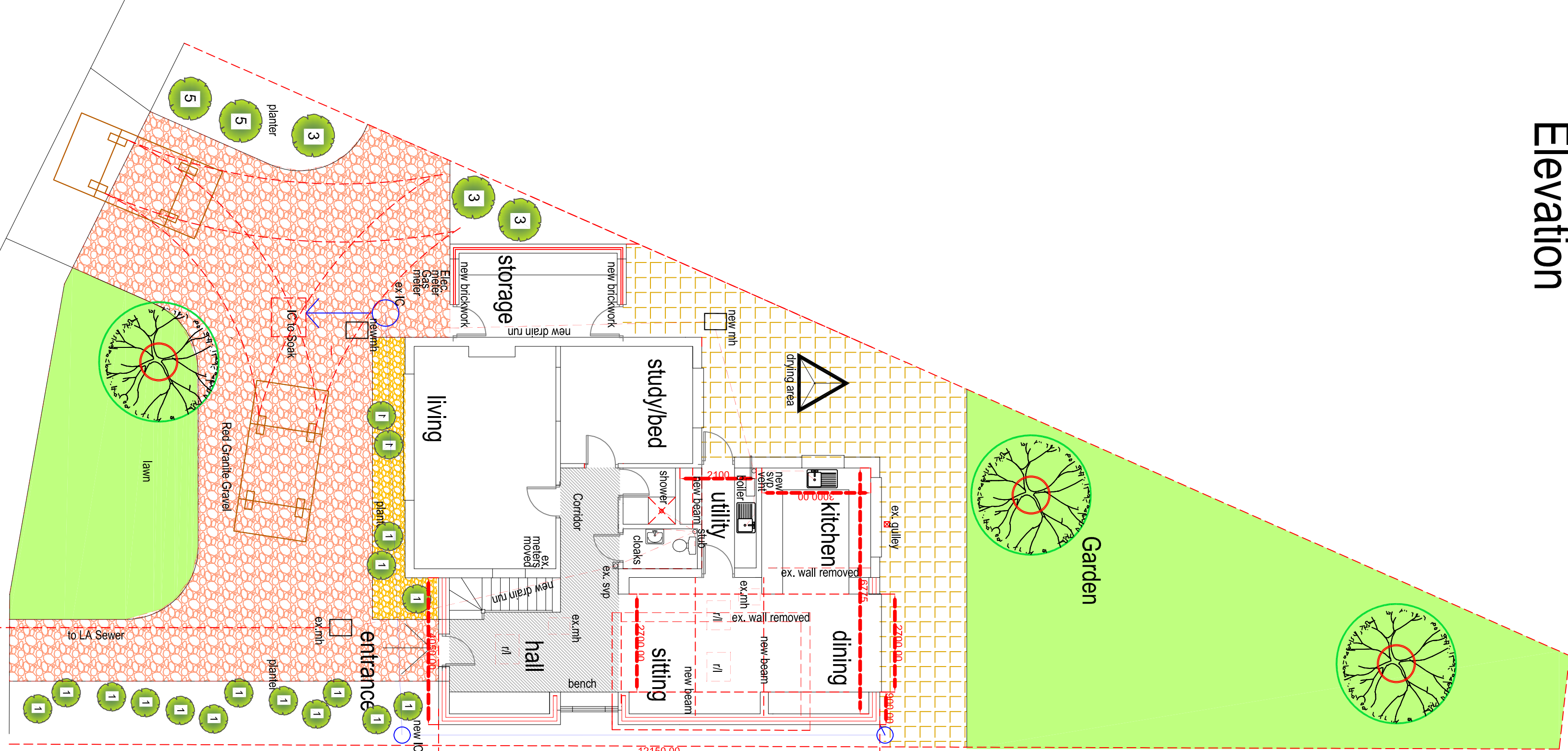
Southbrook Road Proposed Ground Floor and Site Plan
