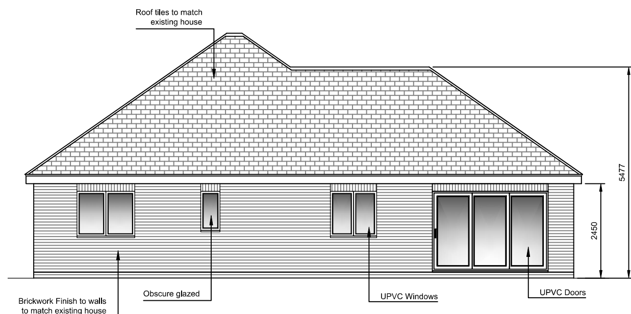
Rear Elevation
