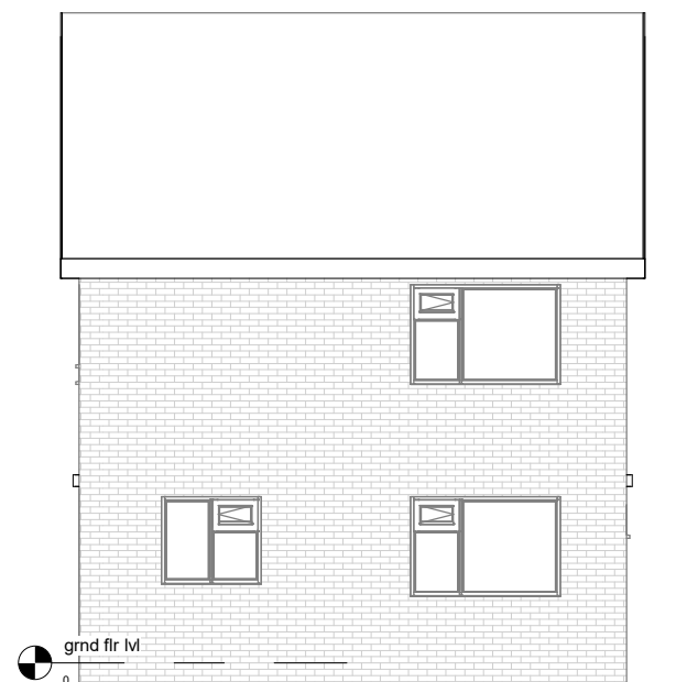
Existing Elevation-Rear
