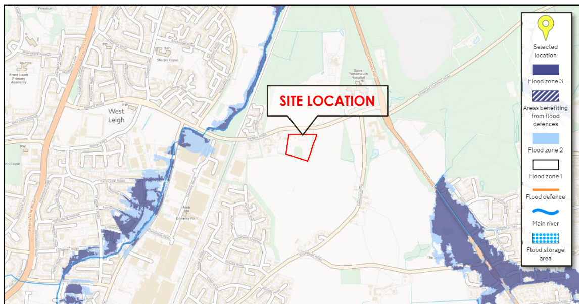
Figure 5.1 - Environment Agency Flood Zone map
