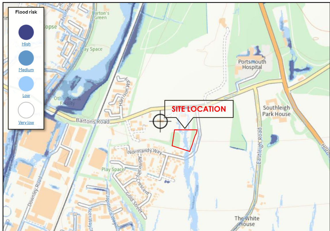
Fig 6.2 – Environment Agency Flood Risk from Surface Water map
