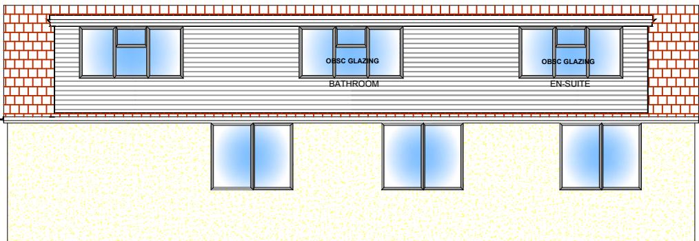
PROPOSED SIDE ELEVATION D
