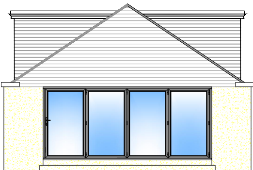
PROPOSED (NEW) REAR ELEVATION C
