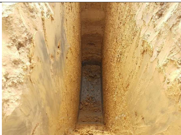
Plate 1 – TP01 – Trial pit
