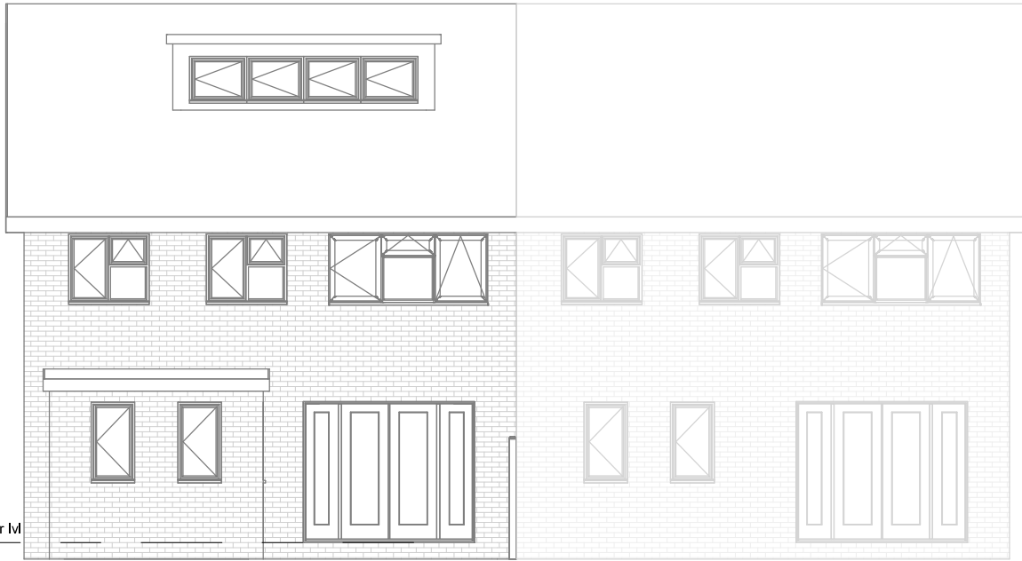
Existing Elevation-Rear
