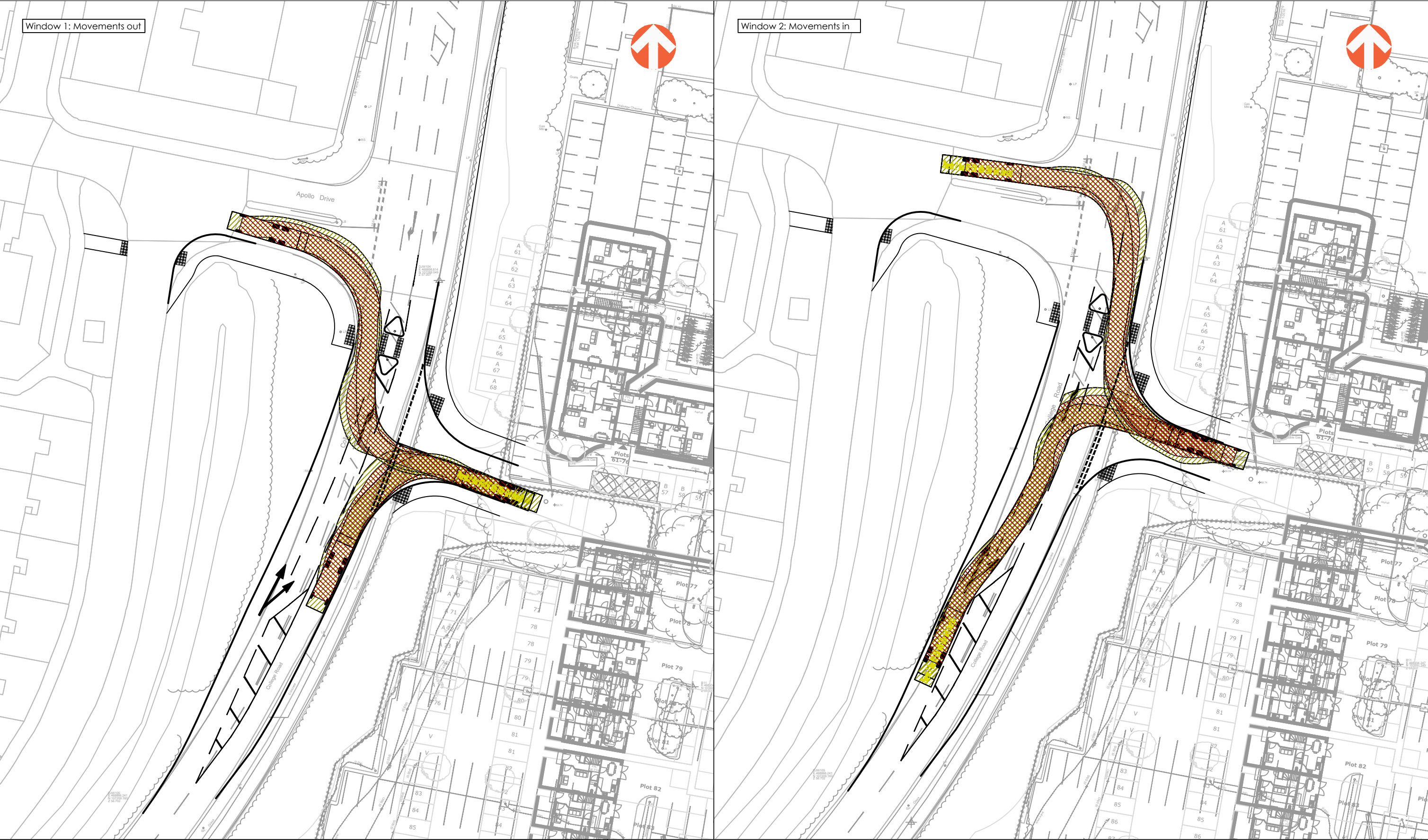
Vehicle profile - 11.2m Refuse lorry
