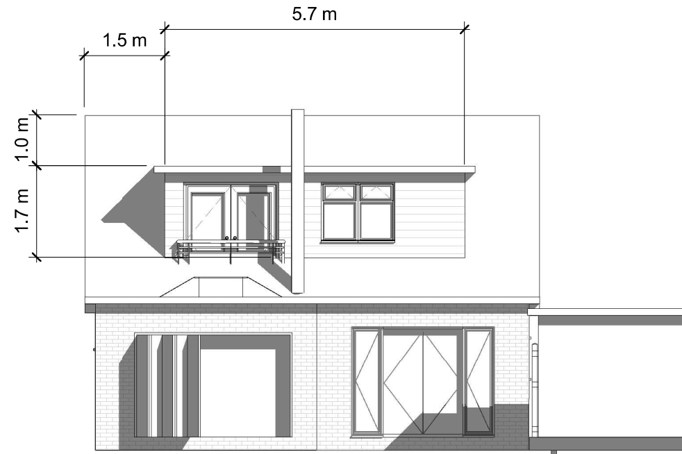
Proposed Elevation-Rear
