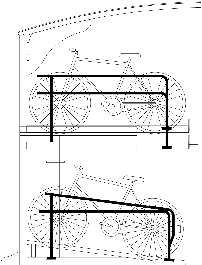
SIDE ELEVATION
