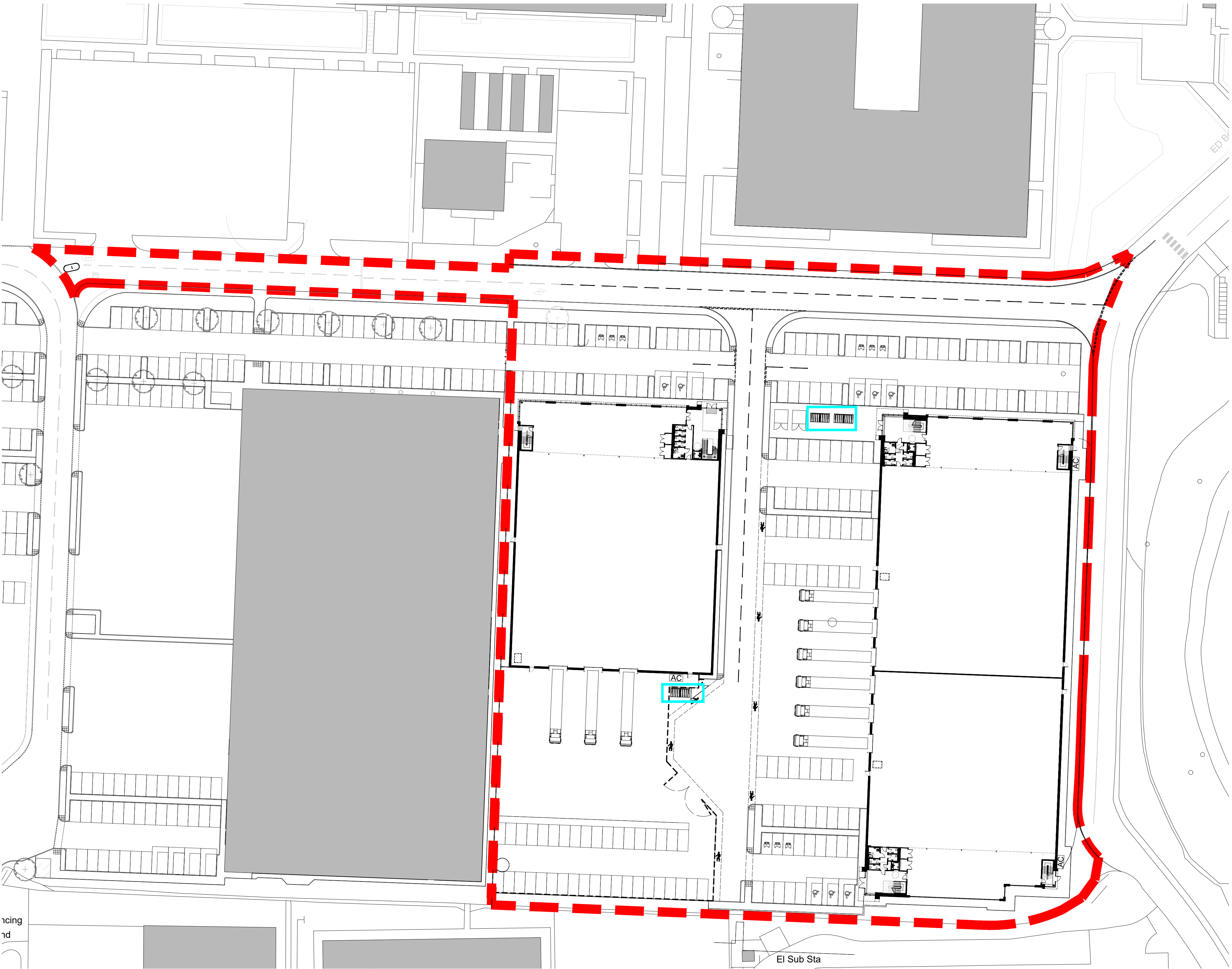
TWO TIER CYCLE STORAGE - FALCOLEVELECO 20 BIKES. RAL 7016 (ANTHRACITE) SHELTER - FALCOGAMMA SINGLE SIDED. RAL 7016 (ANTHRACITE)
