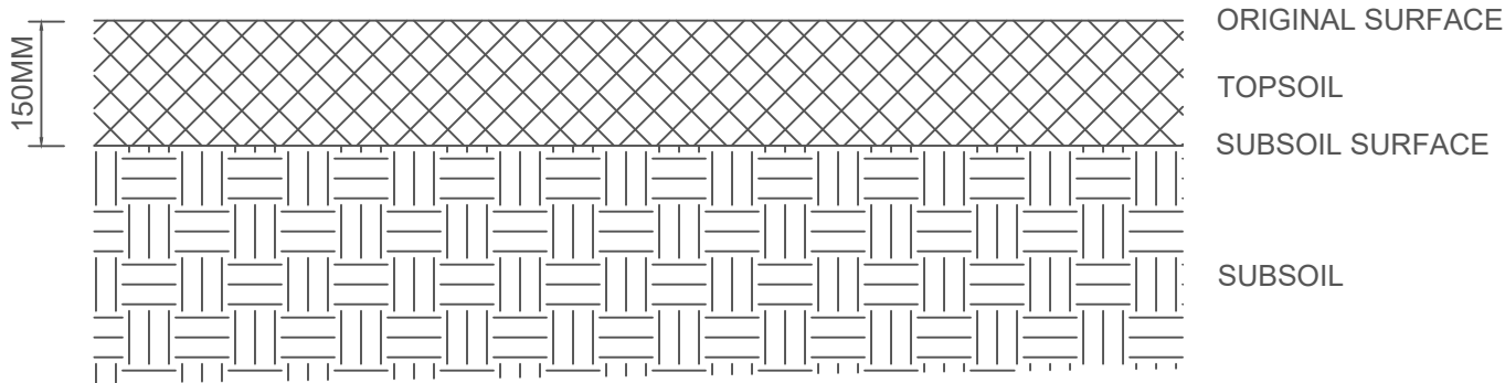
STAGE 1: REMOVE EXISTING TOPSOIL AND STORE
