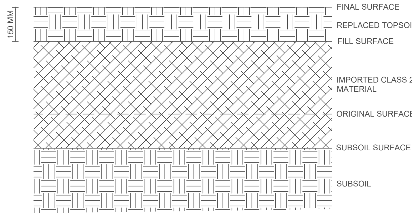
STAGE 3: REINSTATE TOPSOIL FROM STORE
