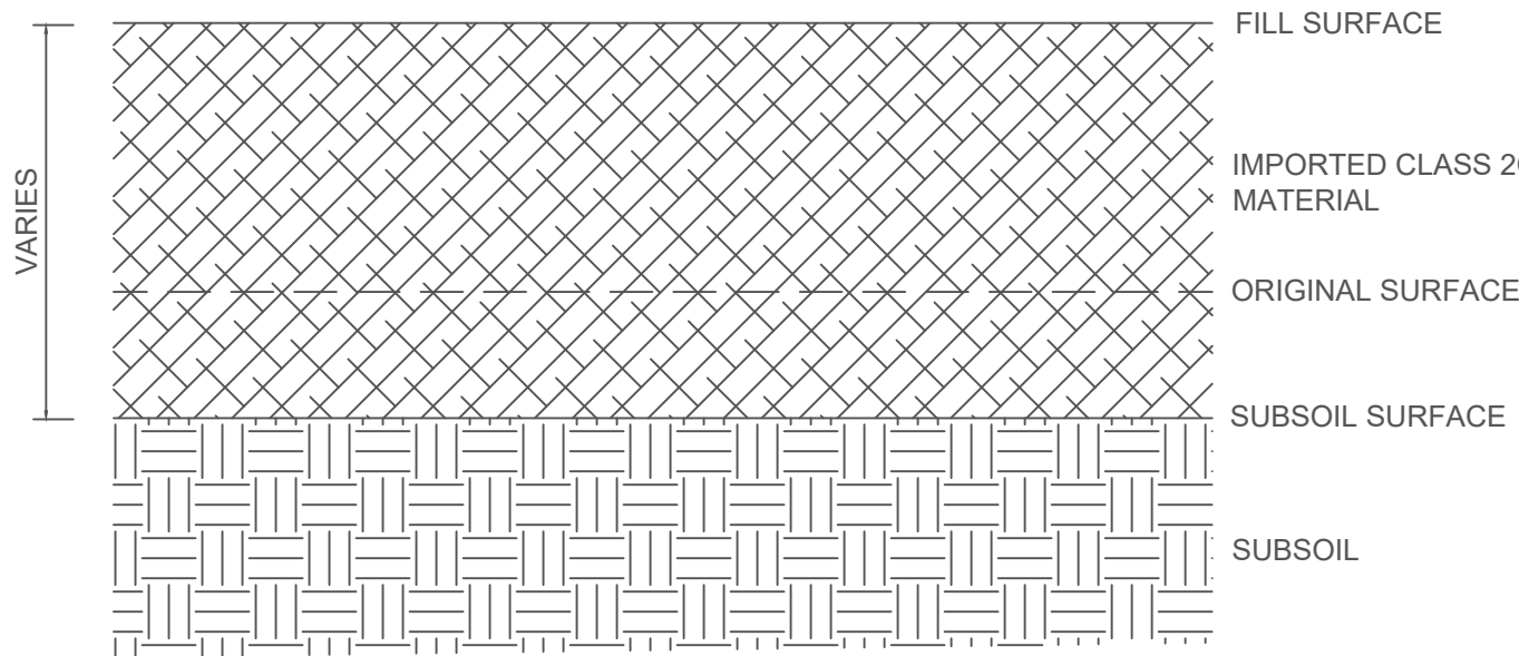
STAGE 2: IMPORT AND PLACE FILL MATERIAL
