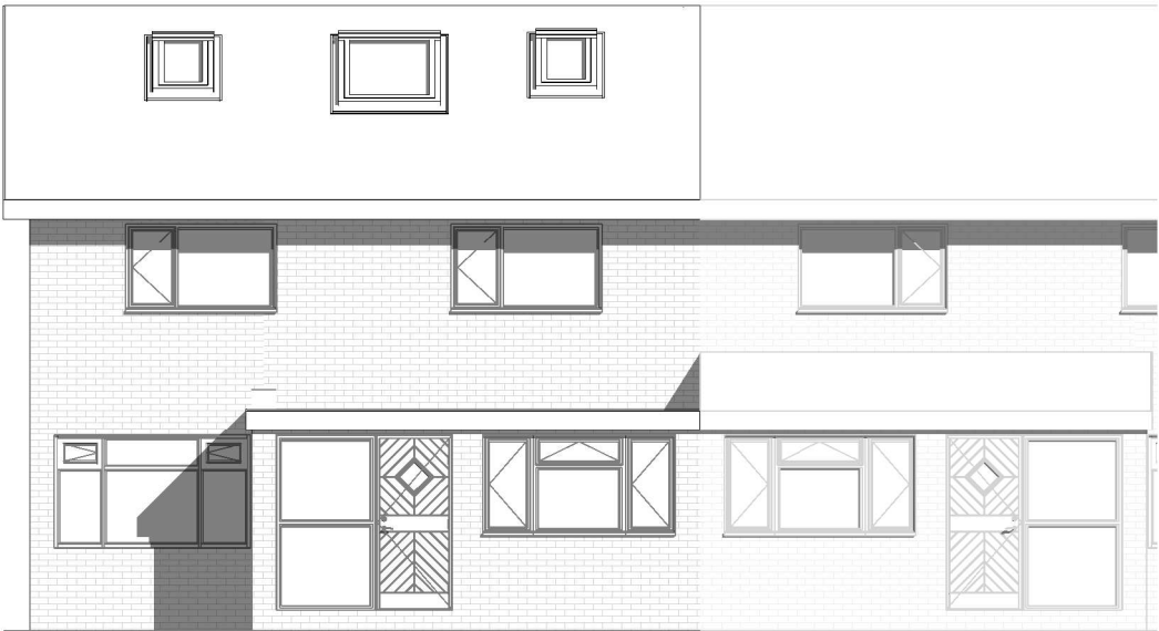
Proposed Elevation-Front
