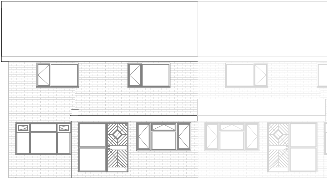
Existing Elevation-Front
