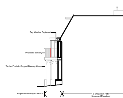
SOUTH ELEVATION 1:100 PROPOSED
