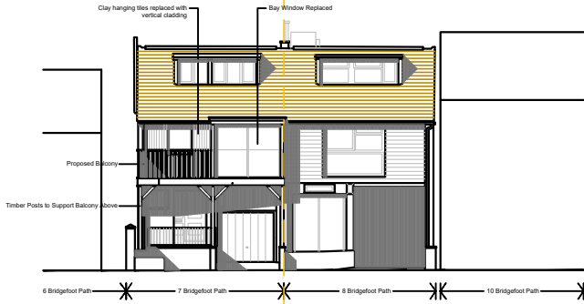
WEST ELEVATION 1:100 PROPOSED
