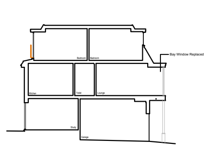
SECTION AA 1:100 PROPOSED
