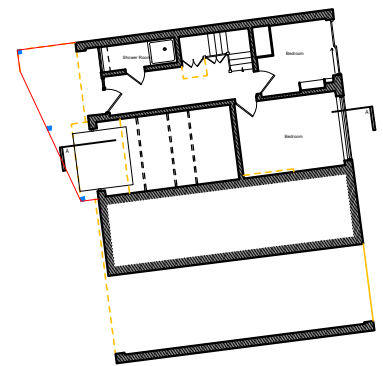
GROUND FLOOR PLAN 1:100 PROPOSED
