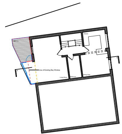
FIRST FLOOR PLAN 1:100 PROPOSED
