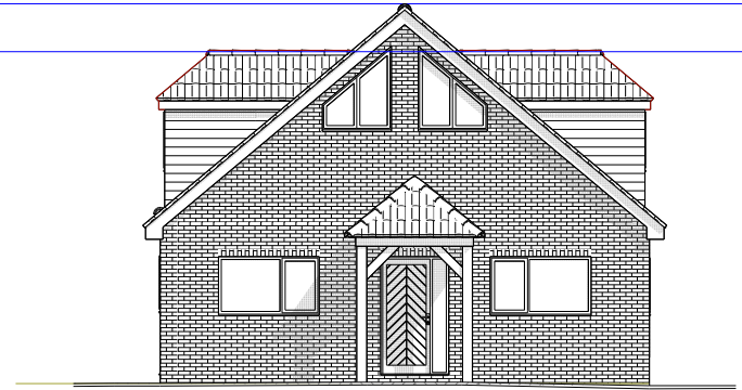
18 Springvale - Front Elevation
