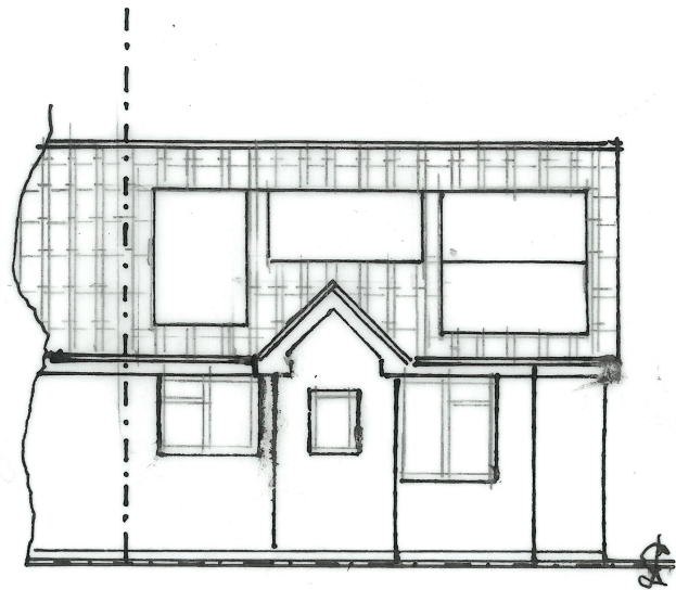
Proposed Front Elevation (west)
