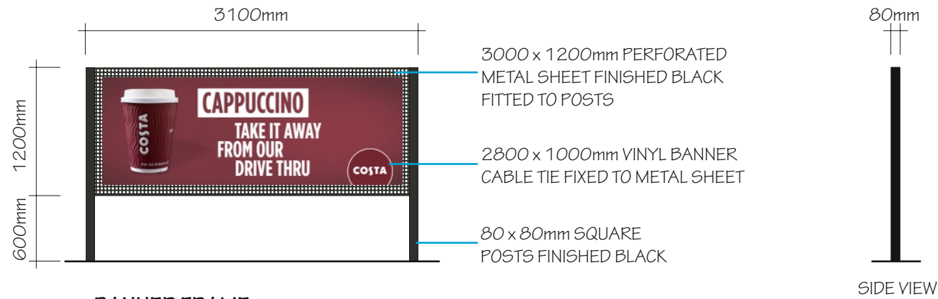
BANNER FRAME NON-ILLUMINATED Scale 1:50
