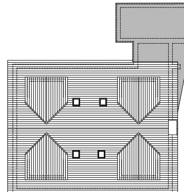
Proposed Roof Plan (Scale 1:100)
