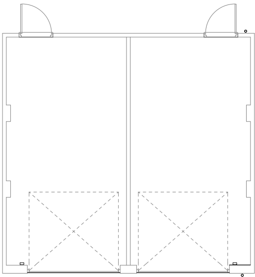
Floor Plan
