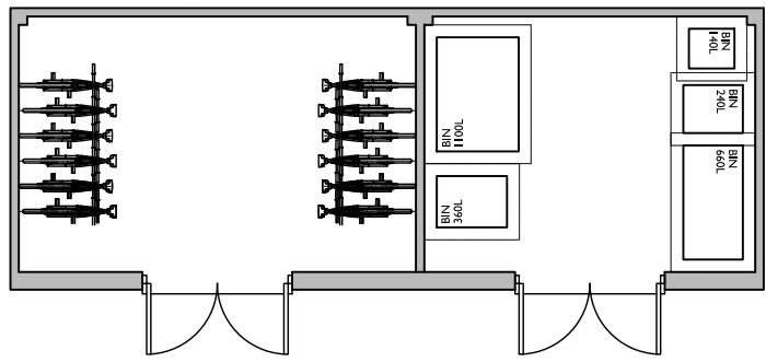
FLOOR PLAN
