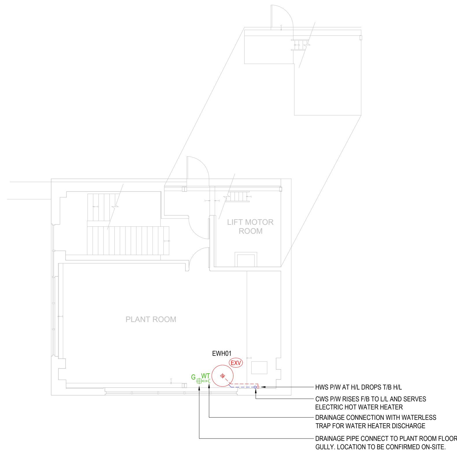
SECOND FLOOR
