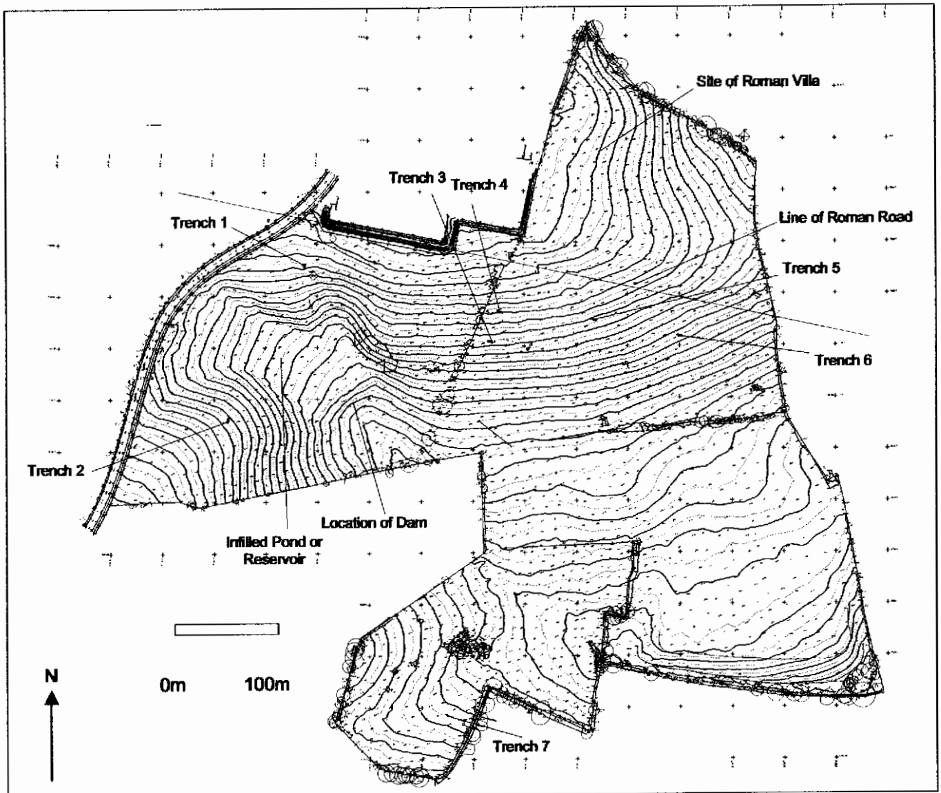
Figure 2. Trench location plan (drawing supplied by Jubb Consulting Engineers Limited)
