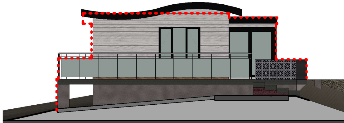
1 East Elevation 1 : 100
