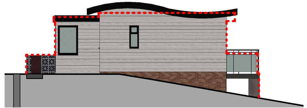
4 West Elevation 1 : 100
