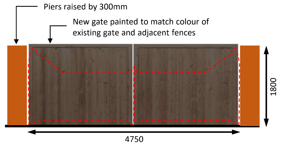
Proposed Elevation
