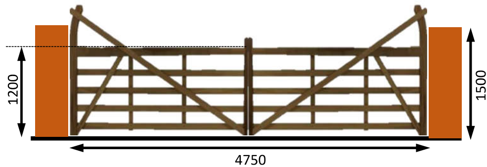
Existing Elevation
