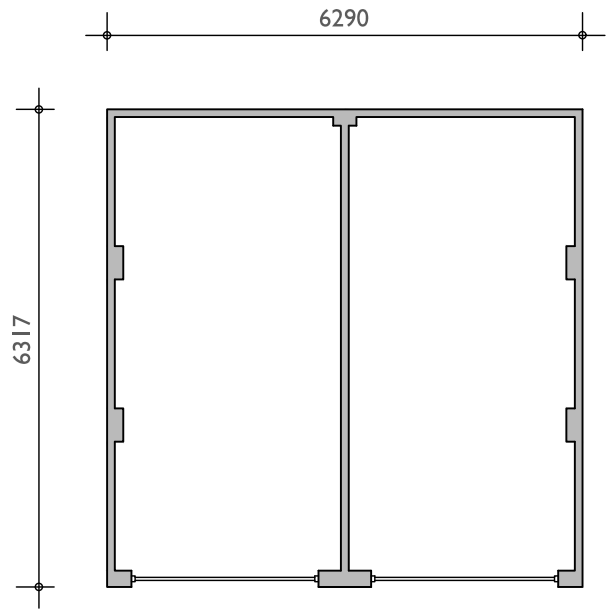
FLOOR PLAN
