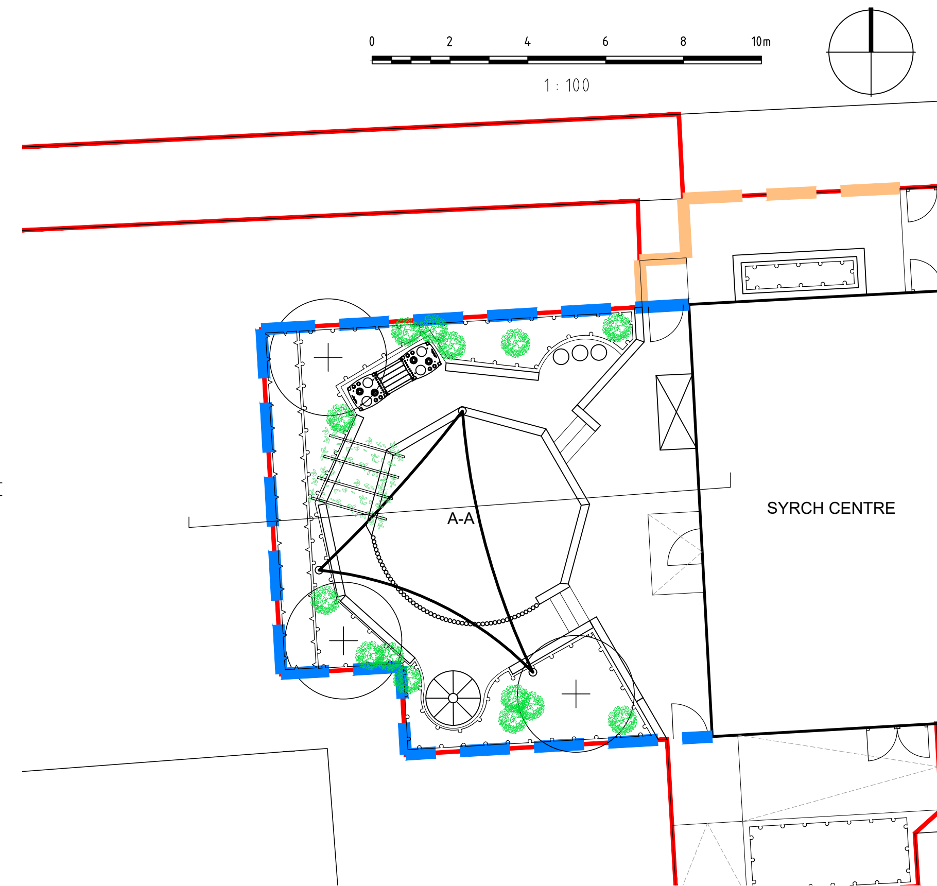
03 Location Plan D01 1:100 @ A1
