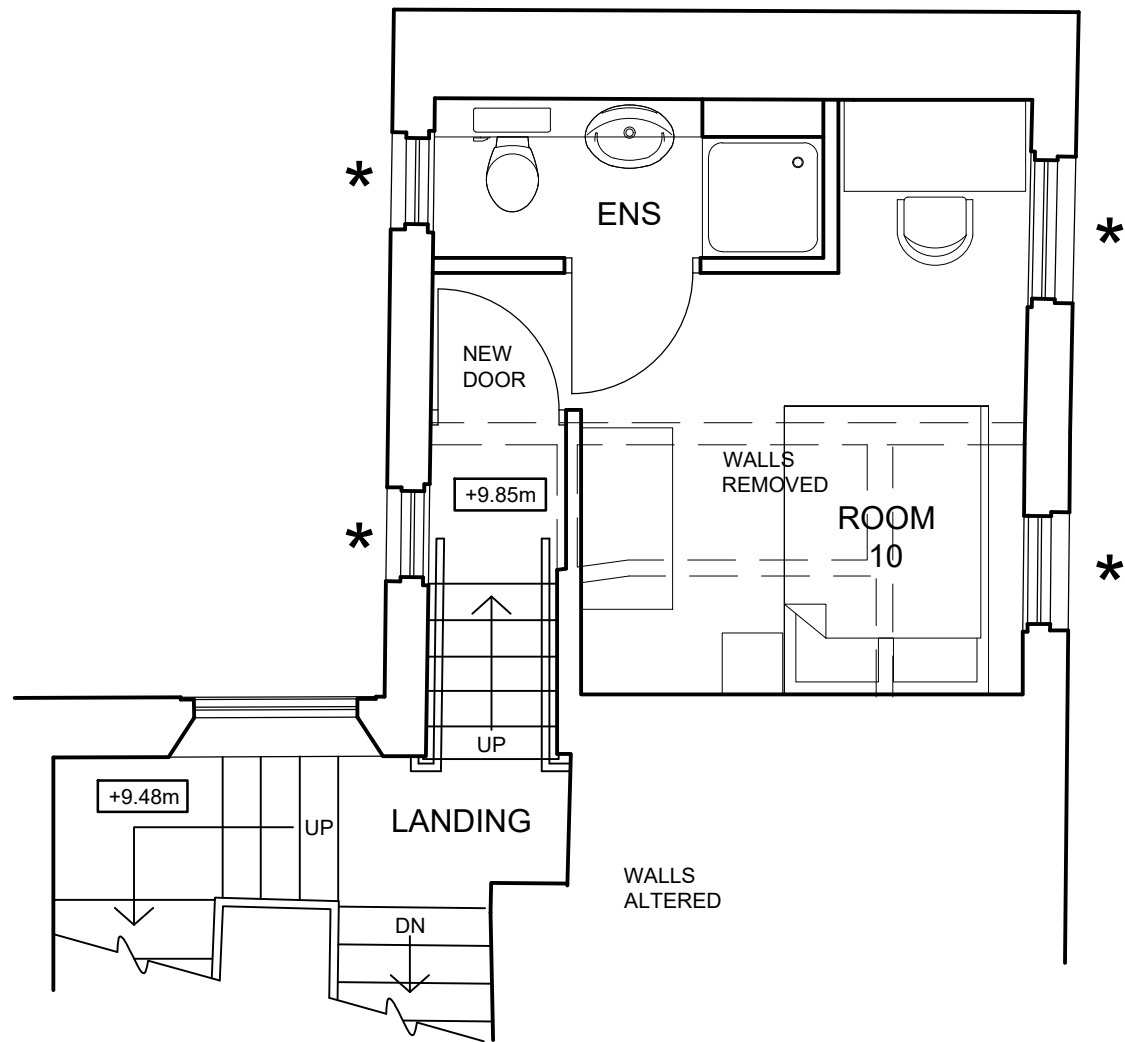
PROPOSED INTERMEDIATE FLOOR PLAN
